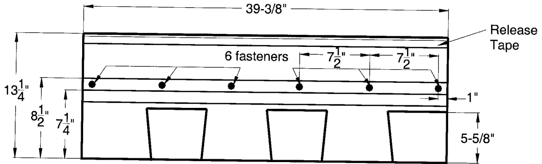
Front Side (Maximum Slope 12:12)
