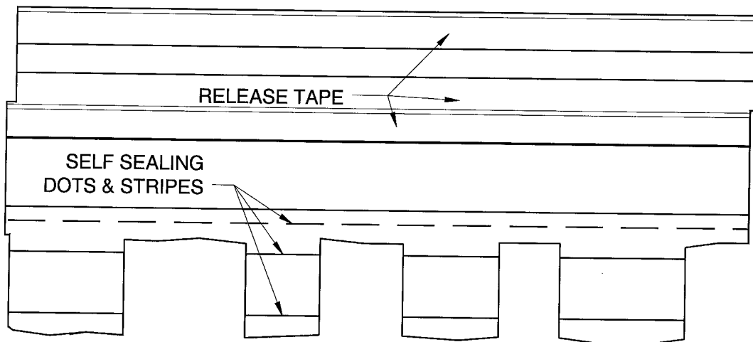
BACK OF SHINGLE
